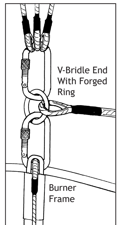
▲ V-Bridle Rigging
