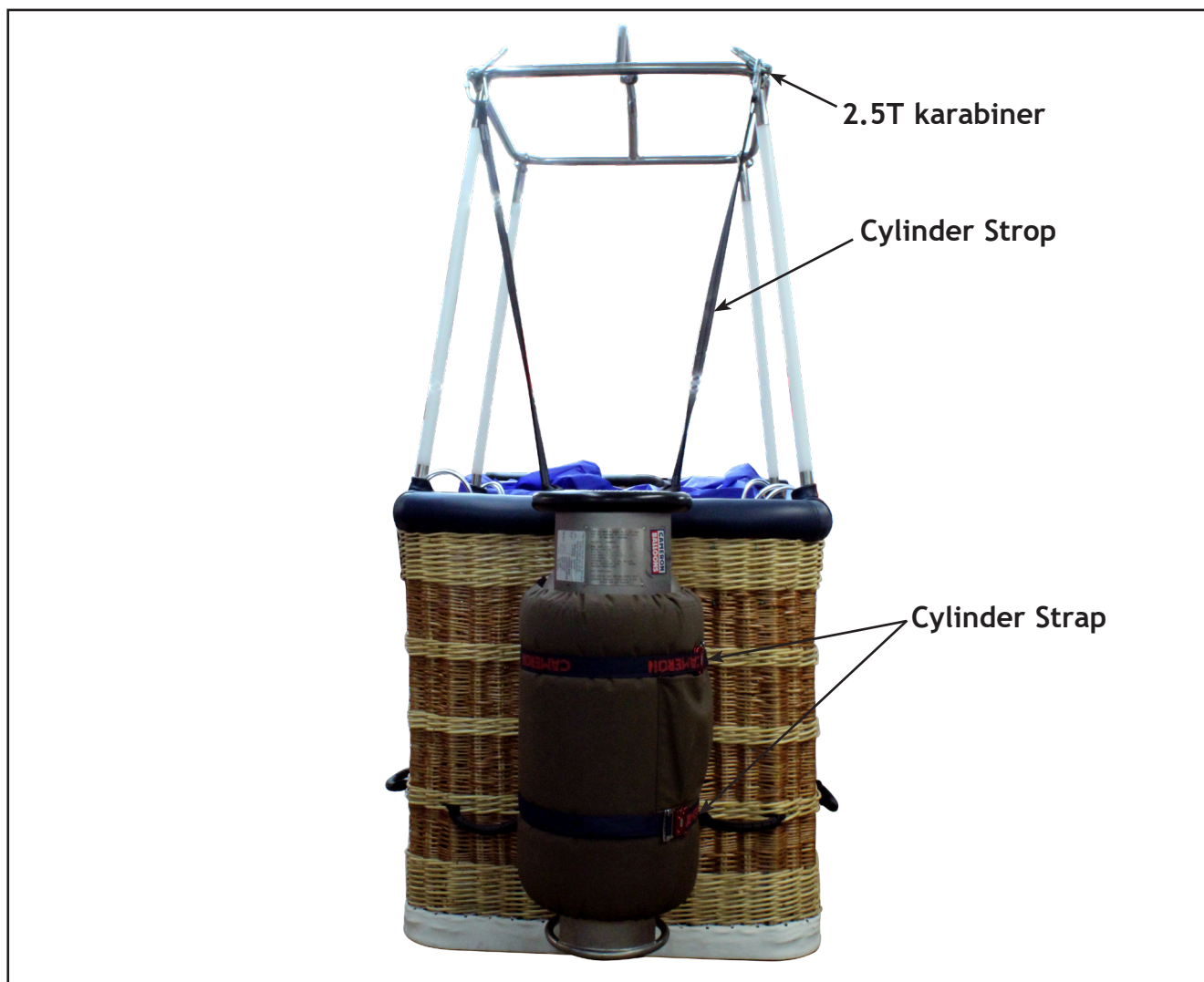
▲ External cylinder arrangement
