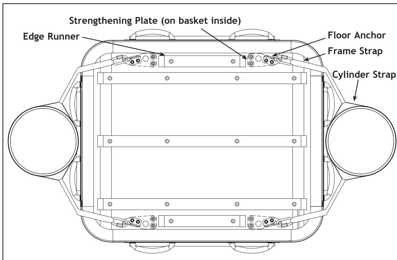
▲ Bottom view of Sportlite Compact external cylinder rigging
