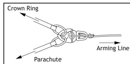
▲ Release Shackle Assembly
