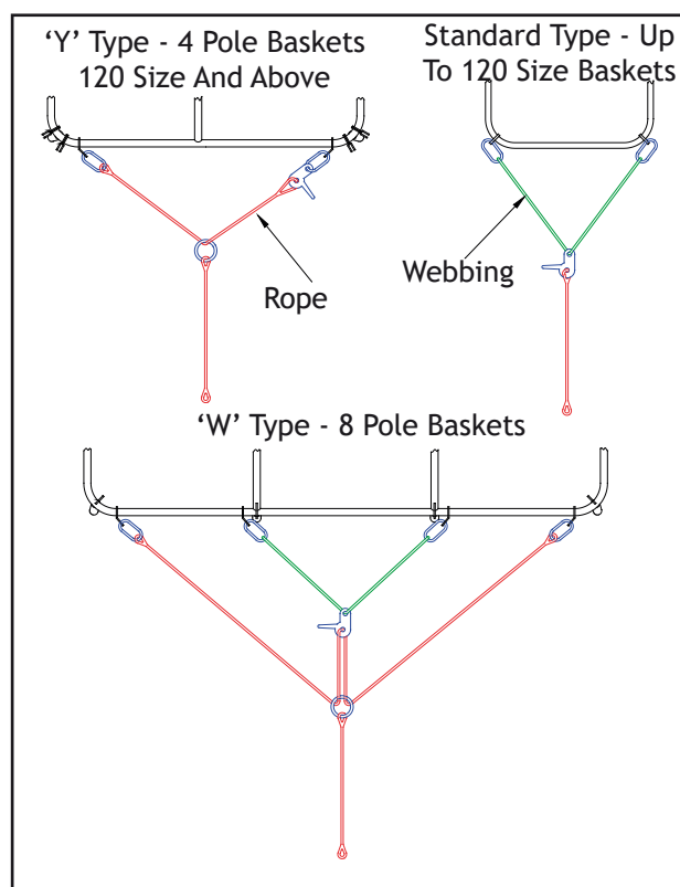
▲ Quick Release Systems
