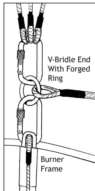
▲ V-Bridle Rigging
