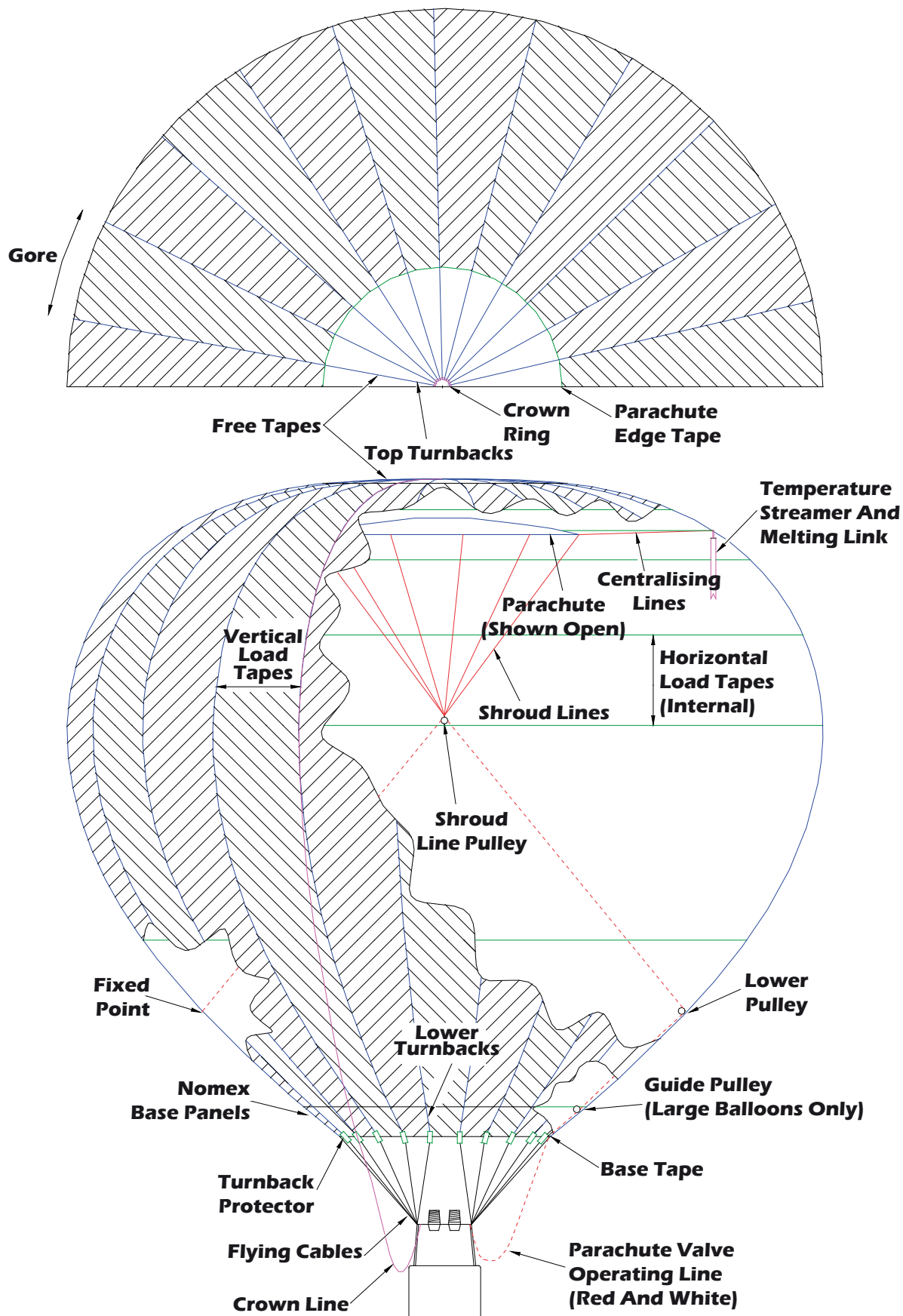
▲ Typical Envelope Description
