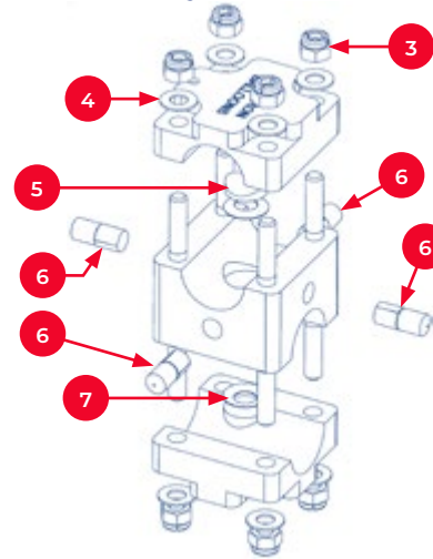
CB-2950-2000 ILLUSTRATED
