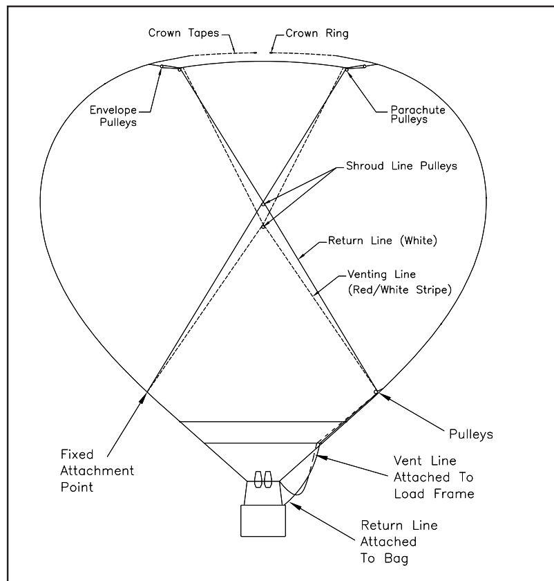
▲ Para Plus Internal Arrangement
