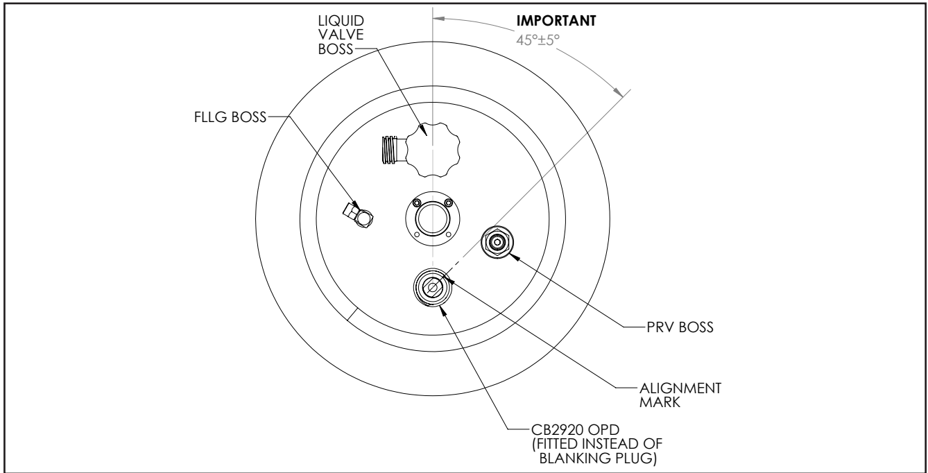
▲ Fig. 3: OPD Alignment Detail
