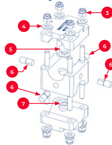
CB-2950-2000 ILLUSTRATED
